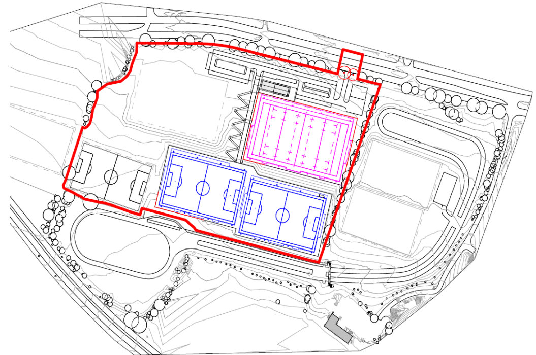
Image 3: Proposed Site Plan
